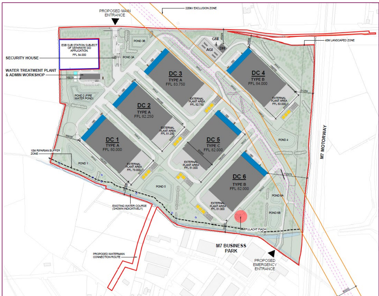
Figure 5.1: Data Centre Application Layout and Planning Boundary
